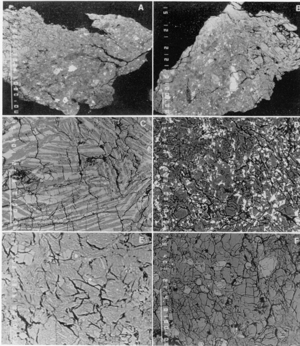
Fig. 2. Photomicrographs of Y-791197,89 taken in backscattered electron mode on the JEOL 733 Superprobe. Shadings represent average atomic number of the minerals, hence plagioclase is dark gray, Fe-rich mafic silicates are lighter, and Fe-rich opaque minerals are bright. Scale bars are shown in the lower left corner of each picture. (A) General texture of subsample 89,1, showing large plagioclase vitrophyre clast. (B) General texture of subsample 89,2 showing large clast of fine-grained feldspathic melt rock. (C) Plagioclase vitrophyre. (D) Feldspathic melt rock. (E) Magnesian melt rock. (F) Granulitic magnesian anorthositic norite.
