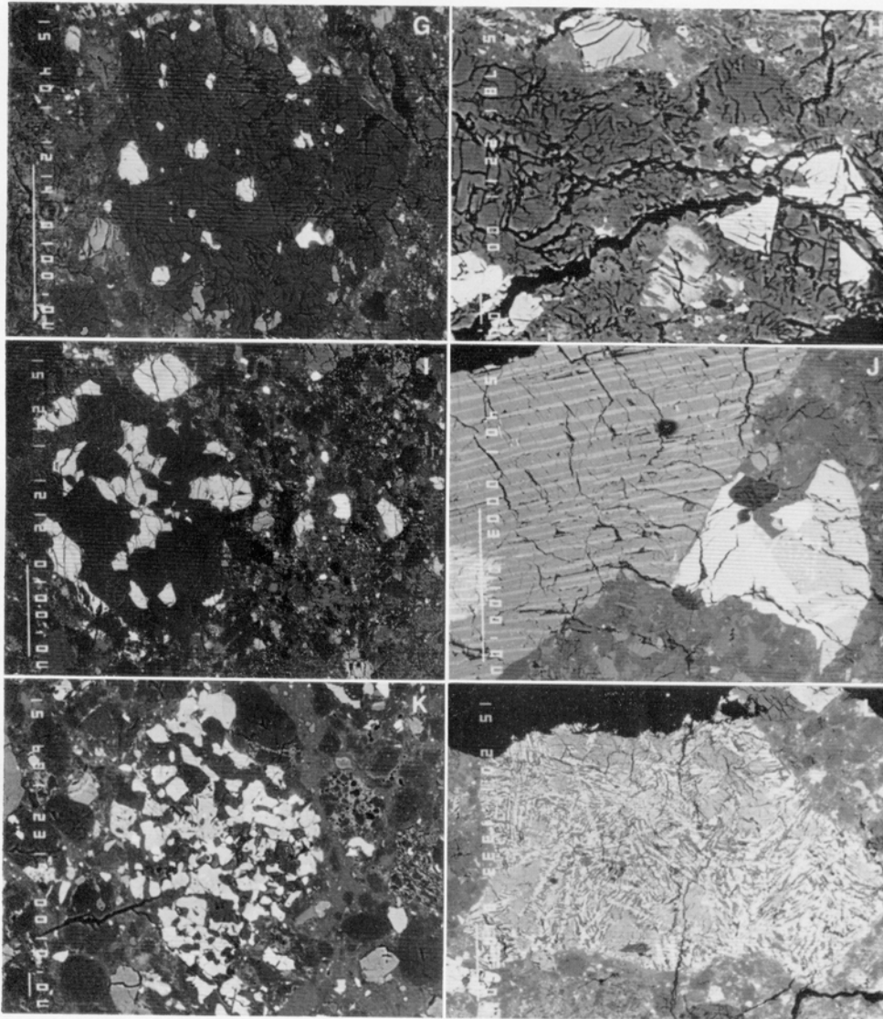
Fig. 2. (continued). (G,H) Ferroan anorthosites. (I) Ferroan anorthositic norite. (J) Highly differentiated assemblage consisting of exsolved clinopyroxene, fayalite, pyroxferroite-hedenbergite, troilite, silica and plagioclase. (K) VLT mare basalt, crystalline. (L) VLT mare basalt, quench-textured.
