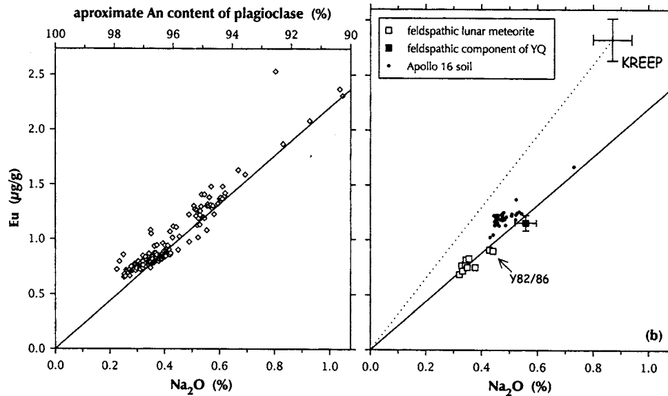
Fig. 7. Variation of Eu with Na 2 O in feldspathic regoliths. (a) Data for 157 highly feldspathic (<2.5% FeO) and KREEP-poor (<1 µg/g Sm) lithic fragments from the Apollo 16 regolith (Jolliff and Haskin, 1995; Korotev, 1997; unpub. data, this lab). The diagonal line ( Eu = 2.20 \cdot Na_2O ) is defined by the origin and the point corresponding to the mean of the data. Points with anomalously low Na 2 O concentrations with respect to the line represent glass spherules or fragments that lost some sodium from volatilization during an impact. (b) The feldspathic lunar meteorites and the feldspathic component of YQ plot along the line (solid) of (a) with Y-82192 and 86032 having higher concentrations than the other feldspathic lunar meteorites. The feldspathic component of YQ has Na 2 O and Eu concentrations more similar to Apollo 16 regoliths than to the feldspathic lunar meteorites. Apollo 16 regolith samples plot off the line to higher Eu concentrations in part because they contain a component of KREEP-bearing impact-melt breccia, which has a greater Eu/Na ratio (dotted line) than plagioclase in highland rocks (Korotev, 1997, 2000).
