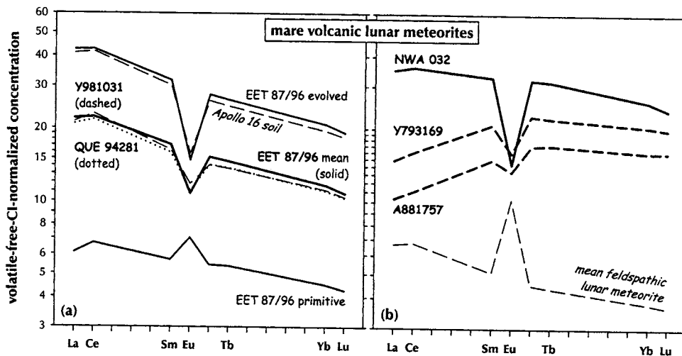
Fig. 5. Concentrations of rare earth elements as a function of atomic number in meteorites from the lunar maria. Meteorites of (a) have relative abundances of trivalent REE that resemble those of KREEP. For reference, data for typical mature regolith ("soil") from Apollo 16 is shown. The Apollo 16 regolith, although feldspathic, derives 82–86% of its trivalent REEs from KREEP-rich impact-melt breccias (Table 8 of Korotev, 1997). As a consequence, it has relative abundances of REE similar to KREEP as well as absolute abundances similar to the meteorites. For EET 87/96, the mean concentrations are shown as well as extreme concentrations inferred for the evolved (high-FeO) and primitive (low-FeO) components (Fig. 3). These compositions were derived from correlations against FeO such as that of Fig. 3b extrapolated to 13.5% and 24.5% FeO, that is, the extremes of the range of the EET 87/96 splits. The mare basalts of (b) have REE abundances that are more typical of mare basalts from the Apollo missions. Most notably, they have lower La/Sm ratios. The NWA 032 data are from Fagan et al. (2002). The REE concentration values were normalized by 1.36 C, where the C values are the "Mean C1 Chondr." values of Anders and Grevesse (1989). The factor 1.36 normalizes to a volatile-free basis, as in ordinary chondrites (e.g., Nakamura, 1974). The plot is based on only the labeled elements, i.e., those determined by INAA. Values for other elements are interpolated, except that Gd (between Eu and Tb) values are estimated (mean of Ce-Sm and Yb-Tb extrapolations).
