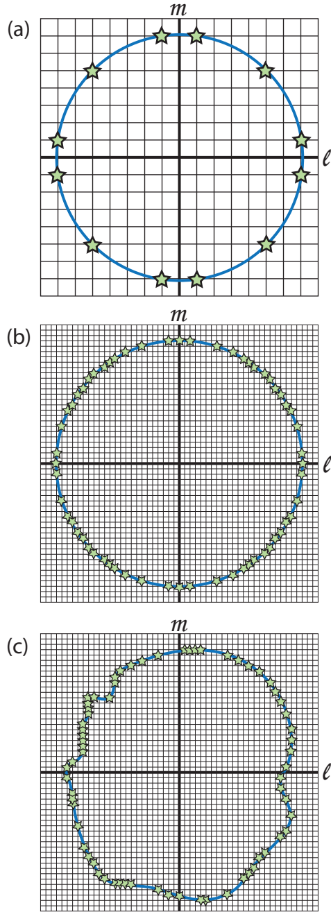
Figure 1. Graphical depiction of solutions for degenerate (traveling wave) modes on a square. Each grid point corresponds to a mode. Intersections of the curve r = \omega_{l,m} L / (\pi c) with grid points denote modes with the same degeneracy (denoted by stars). (a) When r = 5\sqrt{2} , the circle intersects 12 grid points. (b) When r is large, the modes are approximately evenly spaced. (c) When c is not constant, modes are no longer guaranteed to be evenly spaced. Intersections for cases (b) and (c) are approximate.
