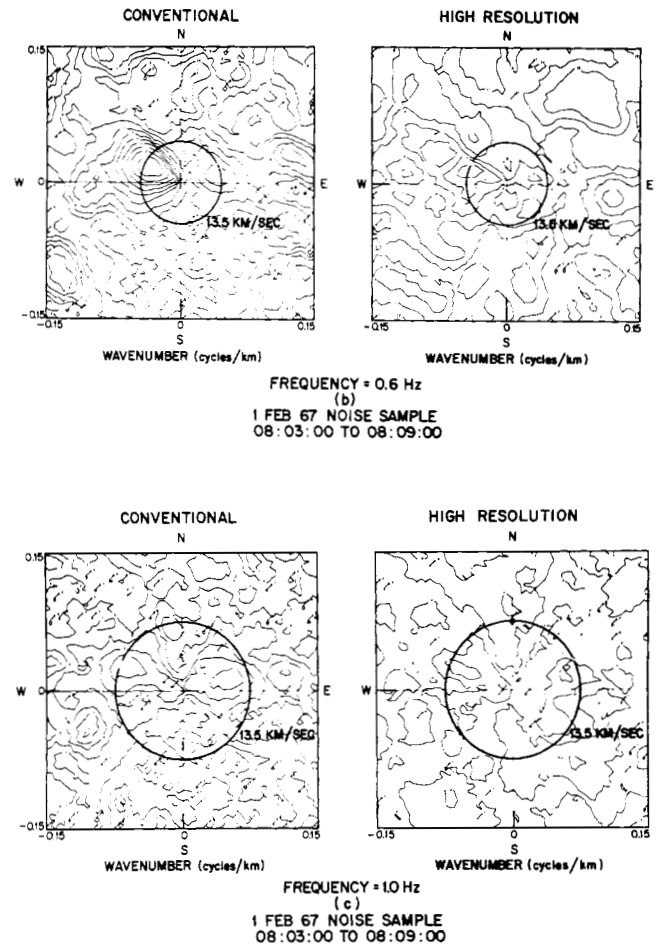
Fig. 10. Conventional and high-resolution frequency-wavenumber spectra for 1 February 1967 short-period noise sample: 08:03:00 to 08:09:00. (a) Frequency=0.2 Hz. (b) Frequency=0.6 Hz. (c) Frequency=1.0 Hz.
