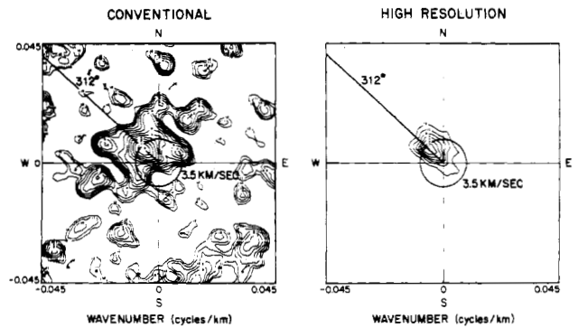
FREQUENCY = 0.03 Hz (a) 21 NOV 66 KURILE ISLANDS EVENT 12:40:00 TO 13:40:00
