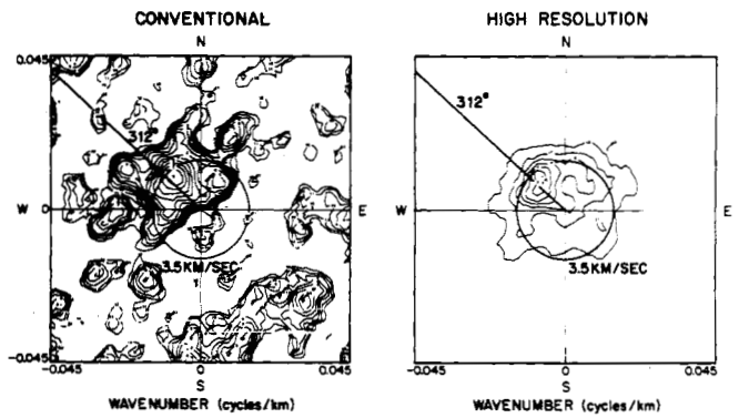
FREQUENCY = 0.05 Hz (c) 21 NOV 66 KURILE ISLANDS EVENT 12:40:00 TO 13:40:00
